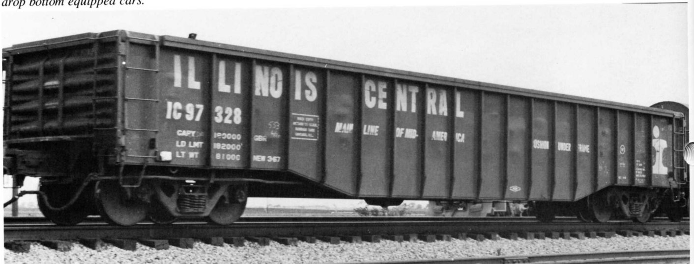
IC 97328 GONDOLA. PHOTO BY BRUCE MEYER - ICHS COLLECTION. The 97300-97349 series 100 ton, 52 ft covered gondolas were built by Greenville in 1967. The cars were equipped with three section removable roofs and assigned to steel service in the Chicago area for loading.
