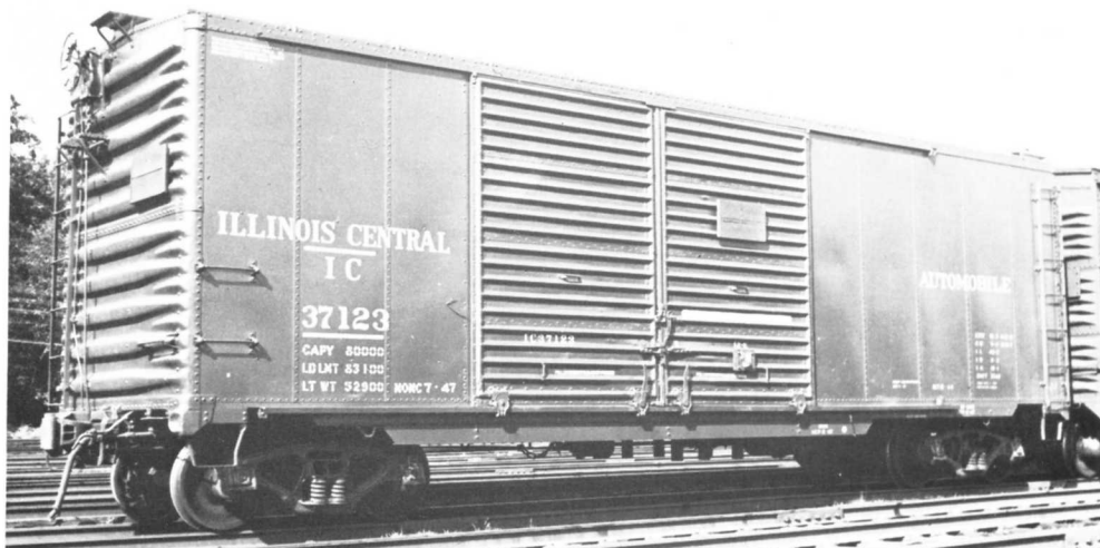
IC 37123 BOXCAR. PHOTO BY G.V. CARSON - DAVID DAISY COLLECTION. The 37000-37499 series cars were built by Mt. Vernon Car Co. in Mt. Vernon, IL in 1940. Cars were equipped with Evans auto loaders that were applied in 1945 and then removed in 1954.
