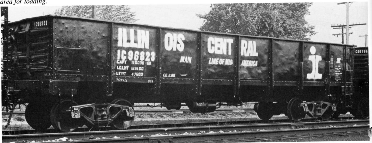
IC 96823 GONDOLA. PHOTO BY ICRR - ICHS COLLECTION. The 96000-96929 series 41 ft, 50 ton solid bottom general service gondolas were rebuilt by the IC Centralia, IL and McComb, MS car shops in 1967 & 1968 from the former 94000-95499 series drop bottom equipped cars.
