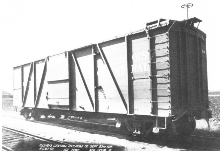
IC 171500 WOODSIDE BOXCAR. PHOTO BY ACF - ICHS COLLECTION.
