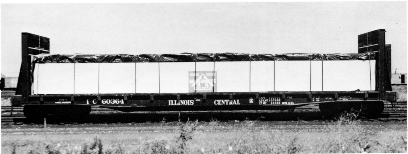
IC 60364 FLAT. PHOTO ICRR - ICHS COLLECTION. The 60300-60470 series cars were built by Bethlehem Steel Co. in 1963. The 50 ton capy bulkhead flats were assigned to wallboard loading.
