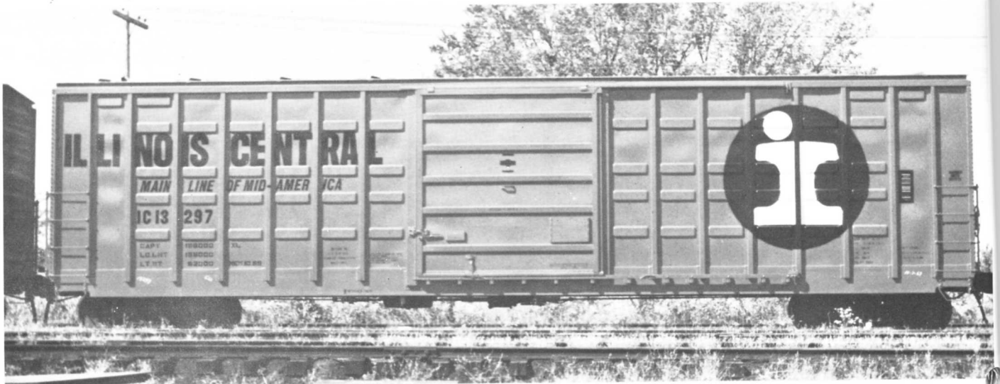
IC 13297 BOXCAR 50FT. PHOTO ICRR CENTRALIA SHOP EMPLOYEES - ICHS COLLECTION. The 13100-13399 series cars were built by the IC Centralia, IL car shop in 1969. Cars equipped with lading strap anchors and 4 belt DF-2 load devices.
