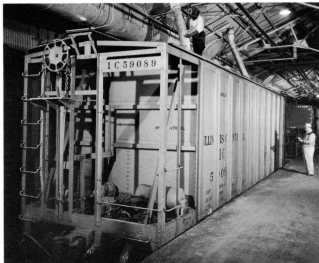
IC 59089 COVERED HOPPER PHOTO ICRR - HE-DRICH-BLESSING - COLLECTION OF ICHS. The 59085-59096 series of cars were built in 1960 by G.A.T.X. and were part of the 59010-59196 single bay airslide covered hoppers owned by the IC. Cars were assigned to flour, sugar and dry chemical service.
