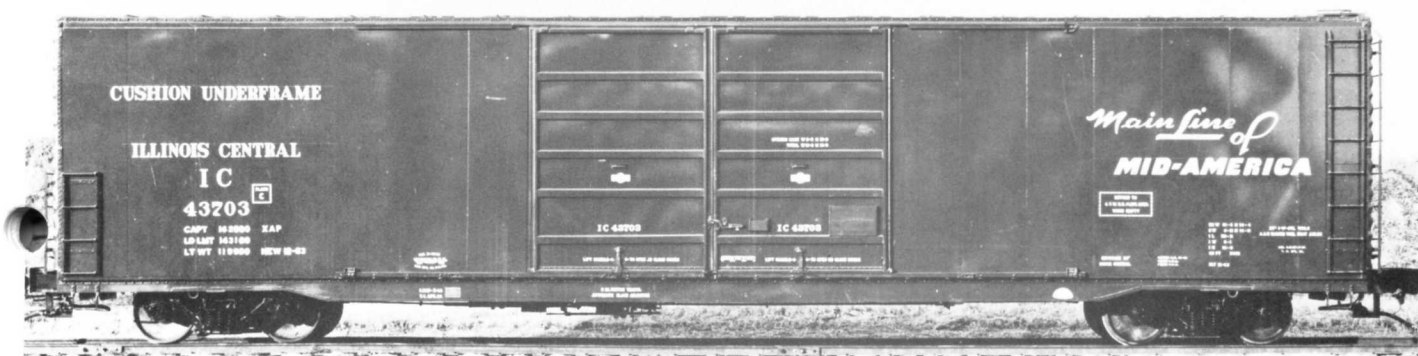
IC 43703 BOXCAR 60FT. PHOTO BY ICRR - DAVID DAISY COLLECTION. The 43700-43749 series cars were built by Thrall in 1963. Cars are equipped with 1/4" nailable steel flooring. Assigned to GTW RR for loading auto axles at Pontiac's Flint, Michigan auto plant.
