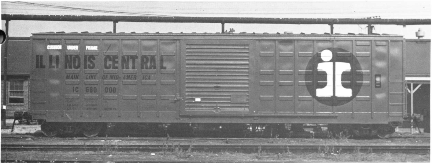
IC 580000 BOXCAR 50FT. PHOTO ICRR CENTRALIA SHOP EMPLOYEES - ICHS COLLECTION. 580000-580399 series cars built by the IC Centralia, IL car shop in 1970. Cars equipped with 4 belt DF-2 load devices and lading strap anchors. 70 ton capy car.
