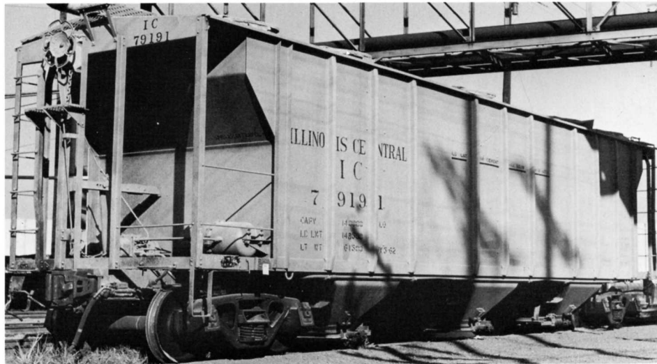
IC 79191 COVERED HOPPER PHOTO ALVINE DOYLE JR. ASSOCIATES, INC. - COLLECTION OF ELLIOT PARKMAN. The 79100-79199 series cars were 70 ton capy built by Pullman Standard in 1955 and were used for cement loading.
