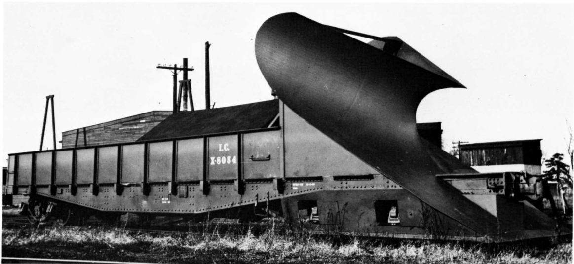
IC X8054 SNOW PLOW. PHOTO G.V. CARSON - ICHS COLLECTION. Part of a group of snow plows that the IC assigned to the northern half of Illinois and the Iowa Division. Converted by the IC from former flat cars, all were built to the same design. Most were equipped with headlights off retired steam engines.
