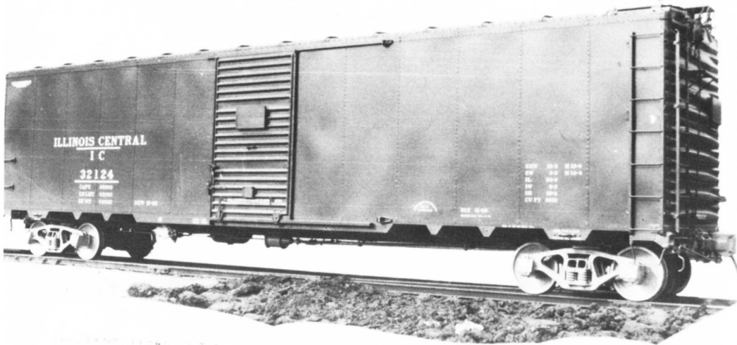
IC 32124 BOXCAR 50FT. SD. PHOTO BY ACF - ICHS COLLECTION. The 32000-32499 series cars were built by ACF in 1940 at their St. Louis, MO plant.
