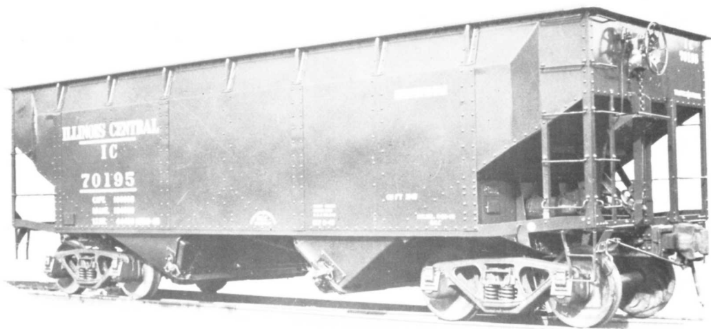
IC 70195 HOPPER. PHOTO ACF - ICHS COLLECTION. The 70000-70499 series cars built by ACF in 1948 in St. Louis, MO. The 50 ton capy cars were assigned mainly to coal service in Southern Illinois and Kentucky.
