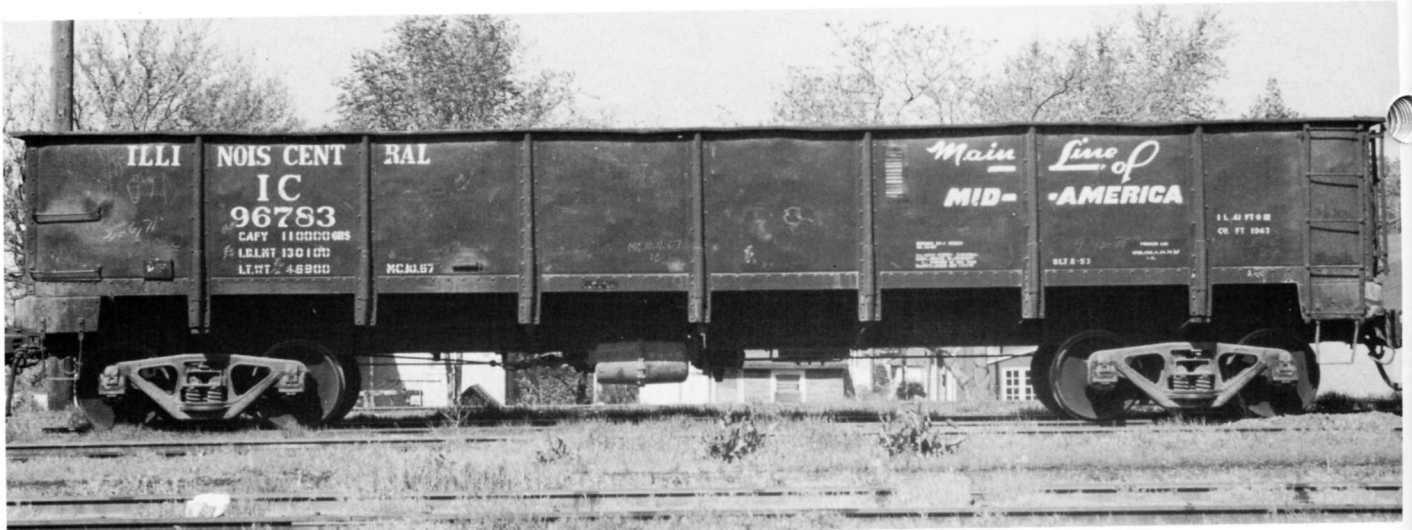
IC 96783 GONDOLA. PHOTO BY BRUCE MEYER - ICHS COLLECTION. The 96000-96929 series 41 ft, 50 ton solid bottom general service gondolas were rebuilt by the IC Centralia, IL and McComb, MS car shops in 1967 from the former 94000-95499 series drop bottom equipped cars.
