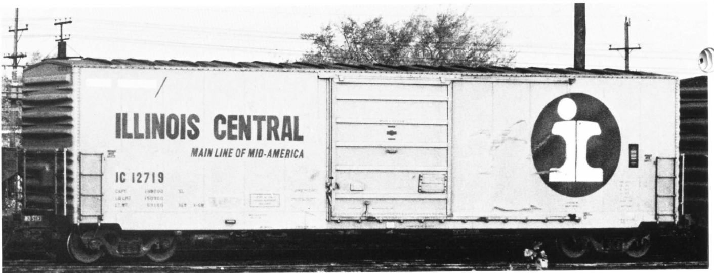
IC 12719 BOXCAR 50FT. PHOTO BY BRUCE MEYER. The 12700-12899 series cars built by G.A.T. Co. in 1968. Cars equipped with SL-2 load dividers and 2 3 / 8 " nailable steel floors.
