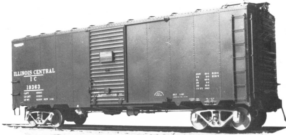
IC 19363 BOXCAR 40FT. PHOTO BY ACF - ICHS COLLECTION. The 19300-19499 series cars built by ACF in 1940.
