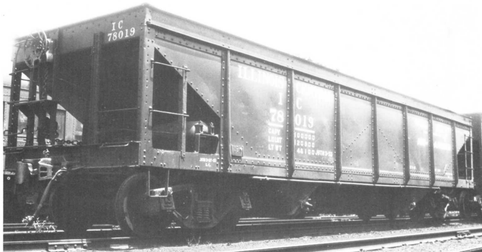
IC 78019 HOPPER. PHOTO G.V. CARSON - ICHS COLLECTION. The 77000-78965 series cars were rebuilt by the IC in 1946 & 1947 from former 90000-93970 hoppers built in 1921.
