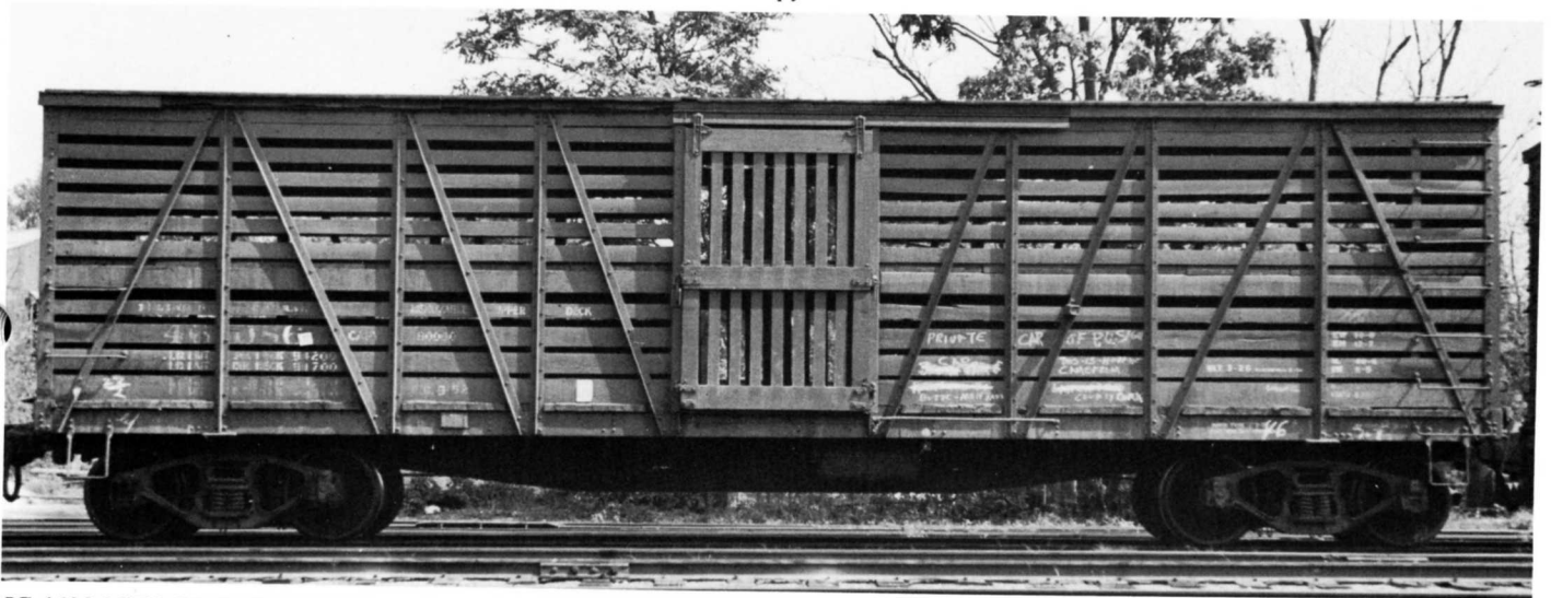
IC 46086 STOCK CAR. PHOTO BY BRUCE MEYER - ICHS COLLECTION. The 46000-46199 were built by General American Car Co. in 1925 & 1926 as 31001-31200 cars. Rebuilt by IC McComb car shops in 1952 and renumbered to 46000-46199 series.
