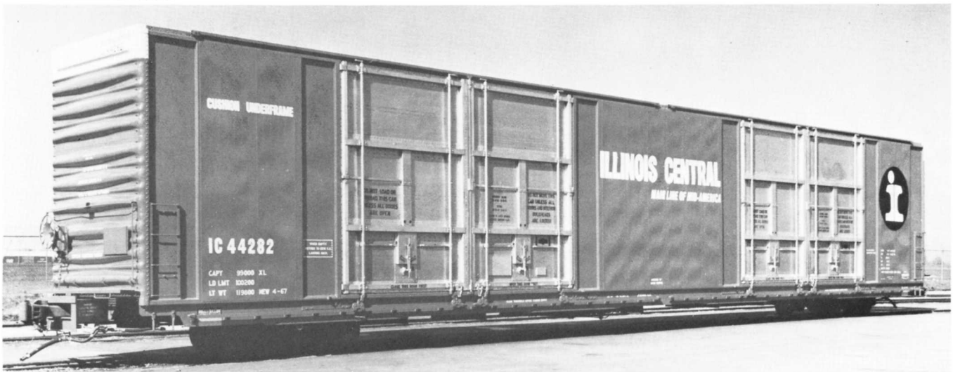
IC 44282 HI-CUBE BOXCAR 86FT. PHOTO ICRR - ICHS COLLECTION. The 44282-44285 series cars were built by Thrall in 1967. Equipped with 2 movable bulkheads and 5 belt rail DF-2 load devices. These cars were assigned to auto parts service.
